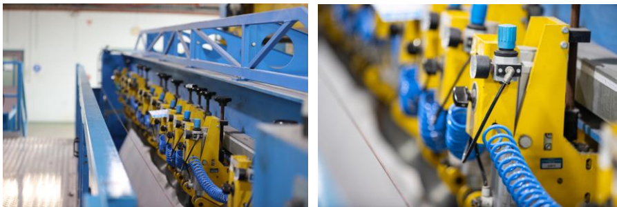
Caption: Compressed air is an essential utility required to operate many functions at Geofabrics - pictured here the in-line slitting process
